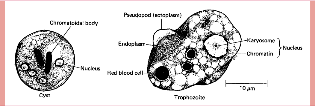
FIGURE 53-1 Entamoeba histolytica .
