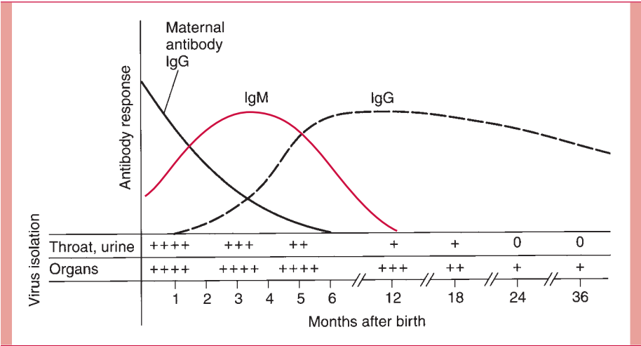
FIGURE 34-2 Persistence of rubella virus and antibody in congenitally infected infants.
