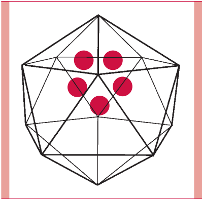
FIGURE 5-4 Diagram of an icosahedron showing 12 vertices, 20 faces, and 30 sides. The colored balls indicate the position of protomers forming a pentamer on the icosahedron.
