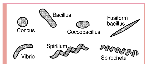
FIGURE 2-2 Shapes of some different bacteria.
