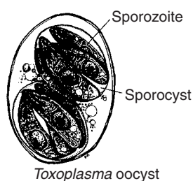
Toxoplasma oocyst
