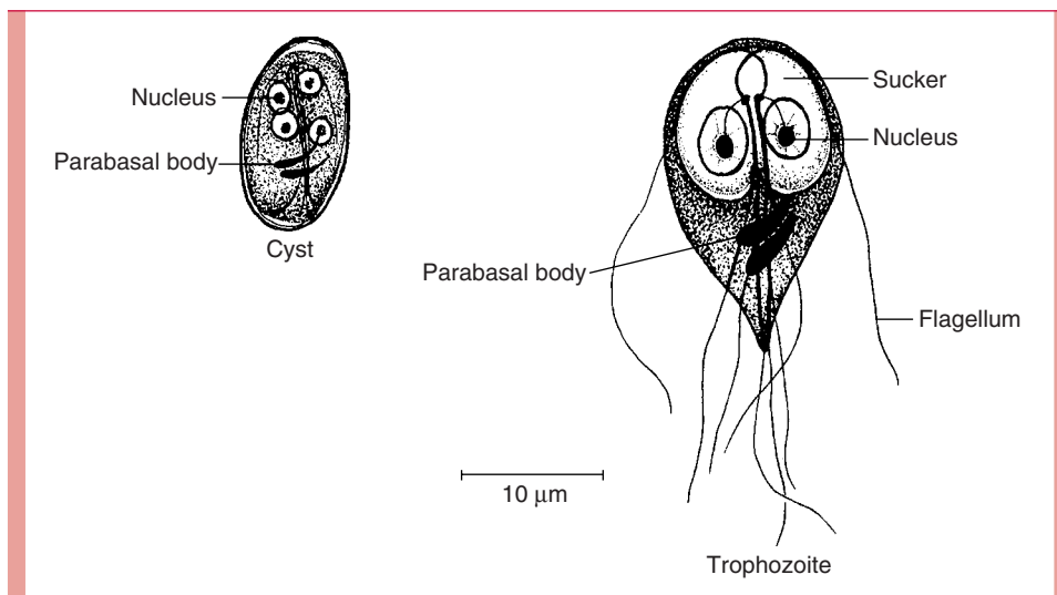
FIGURE 54–2 Giardia lamblia .
