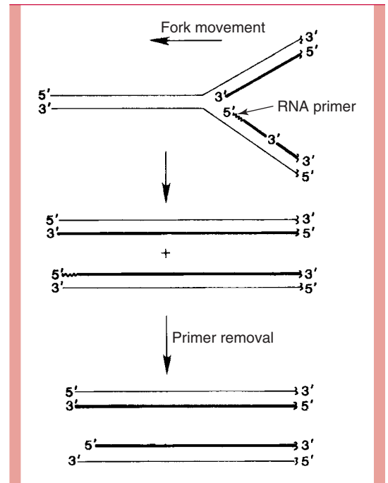
FIGURE 6-7 The end problem in DNA replication.
